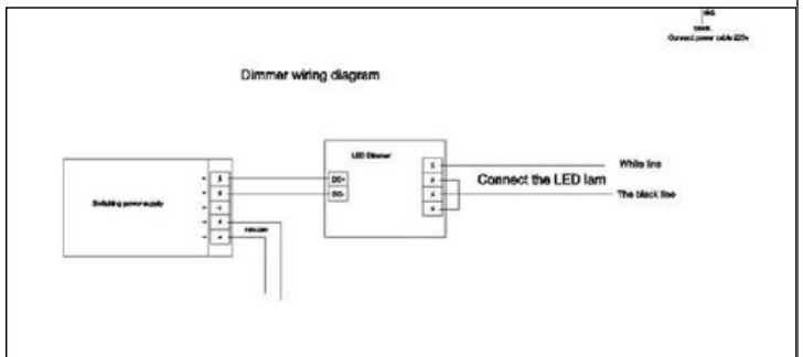
Remote control installation instructions
