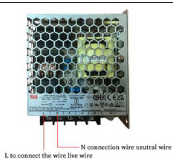
Electrical connection instructions
